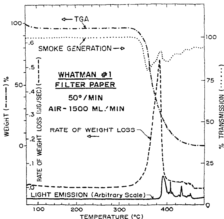
Fig. 2. TG/photometry of Whatman No. 1 filter paper.
